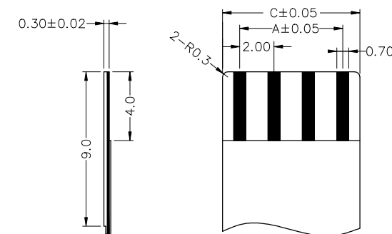
PROPER CABLE (SCALE 2:1)
