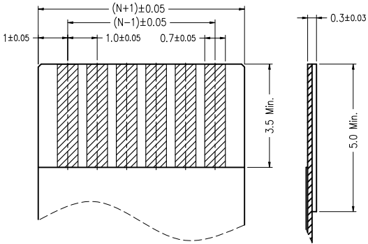
Applicable Flat Cable
