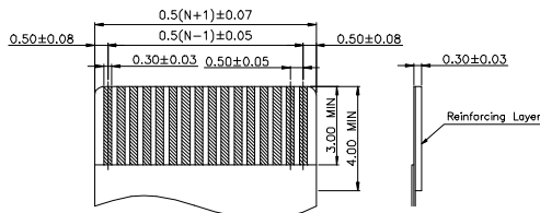
RECOMMENDED FFC DIM
