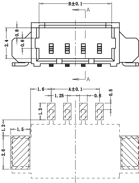
PC BOARD LAYOUT
