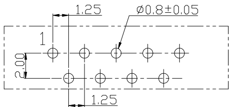
RECOMMEND PCB LAYOUT COMPONENT SIDE (FOR GS15-XX0XA)
