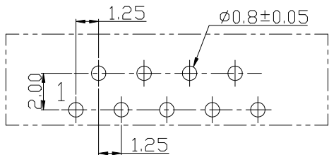
RECOMMEND PCB LAYOUT COMPONENT SIDE (FOR GS15-XX0XAW)
