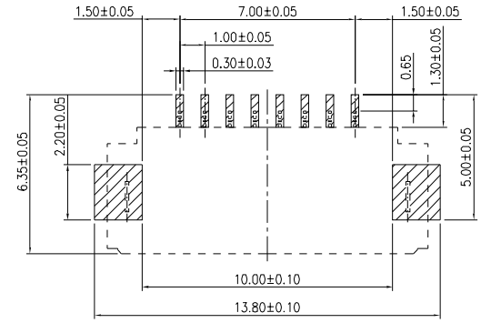
RECOMMENDED PCB LAYOUT GENERAL TOLERANCE ±0.05 / T=0.12
